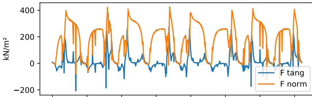
Calculation airgap 1, No Skewing, Rotor position 0.0
